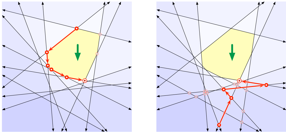
Figure I.1. The primal simplex (falling marble) and dual simplex (rising bubble) algorithms in action.
